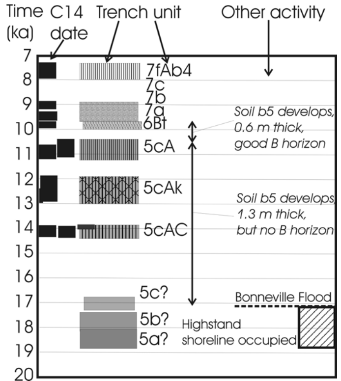
Figure 8. Calibrated C-14 ages (black boxes along vertical axis) from the “pre-colluvial” part of megatrench stratigraphy, compared to Lake Bonneville fluctuations and soil development. Box height represent 2-sigma age range. If unit 5c represents regressive sands from the Bonneville Flood, then soil b5 required about 6,500 years to form, compared to about 1,000 years for soil b4.
