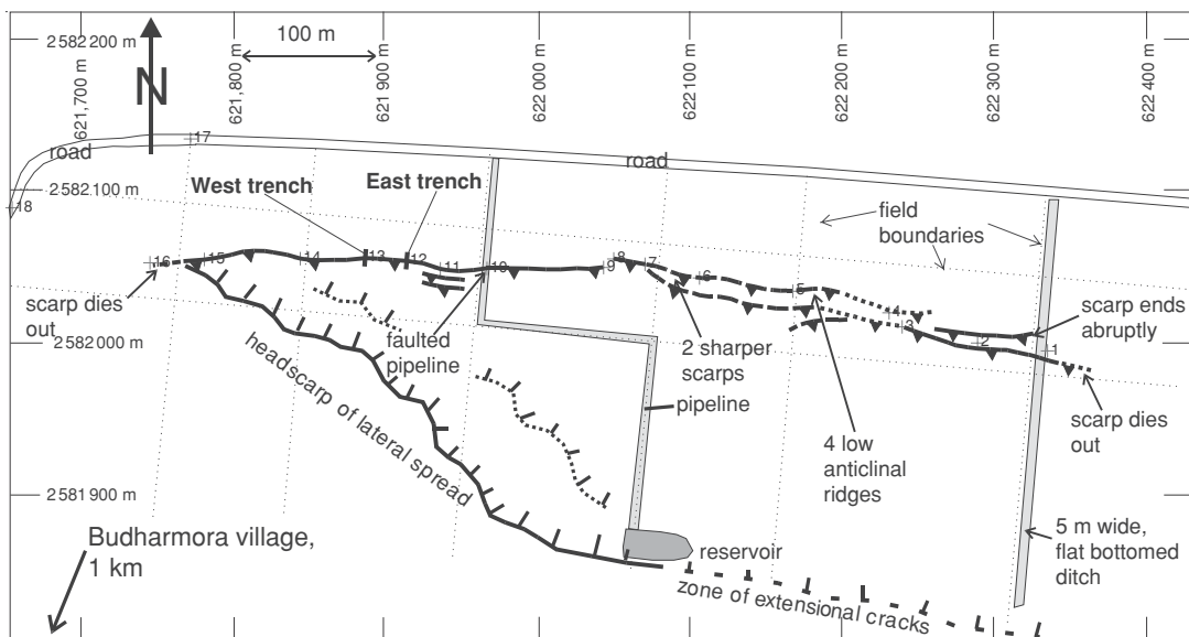
Fig. 16. Reconnaissance GPS map of the lateral spread north of Budharmora village. Coordinates are UTM meters, Zone 42, WGS84 datum. Thick black lines show the margins of the spread, with hachures indicating extensional scarps and teeth indicating compressional scarps or anticlinal ridges. The log of the west trench across the toe thrust is shown in fig. 17. Both extensional and compressional scarps die out to the east.
