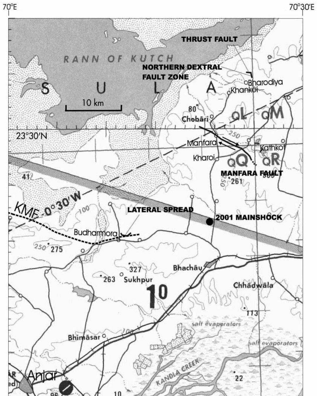
Fig. 2b. Detailed map showing location of 2001 surface faulting and lateral spreading (thicker gray lines with associated bold labels). KMF = Kachchh Mainland Fault.
